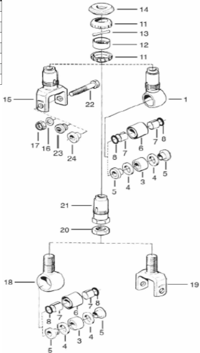
End eye
