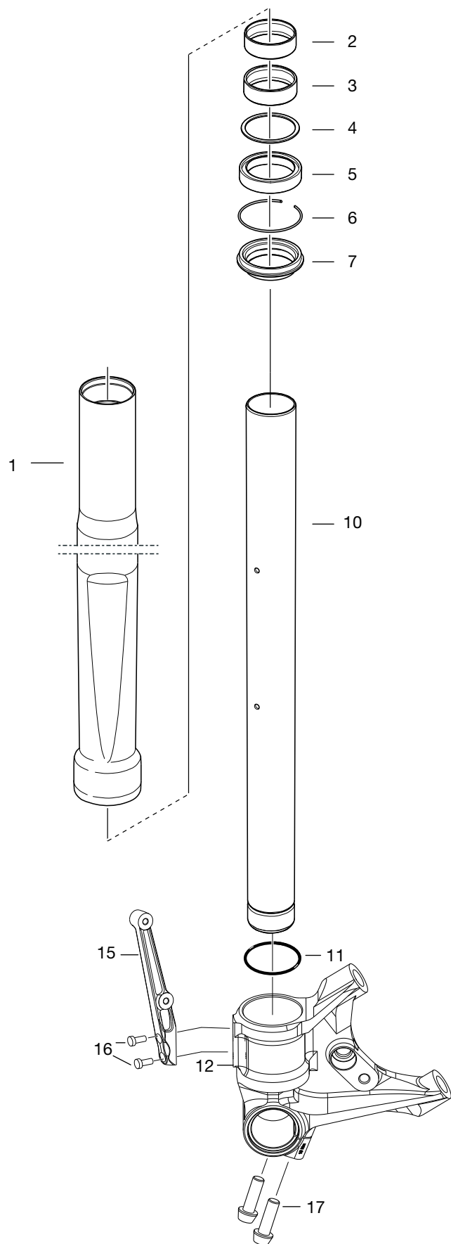
Figure 2 - External Components
