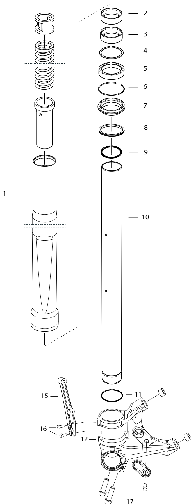
Figure 2 - External Components
