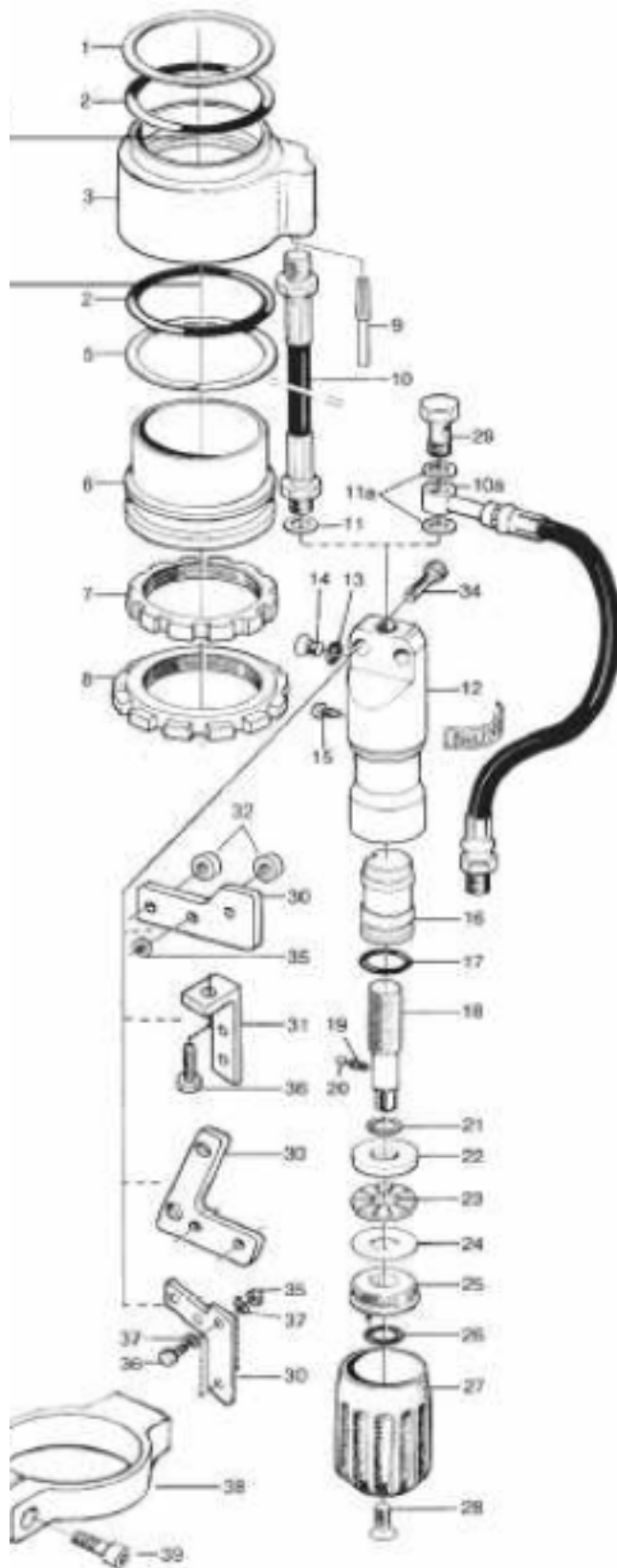
Fig.4 Preload housing assy
