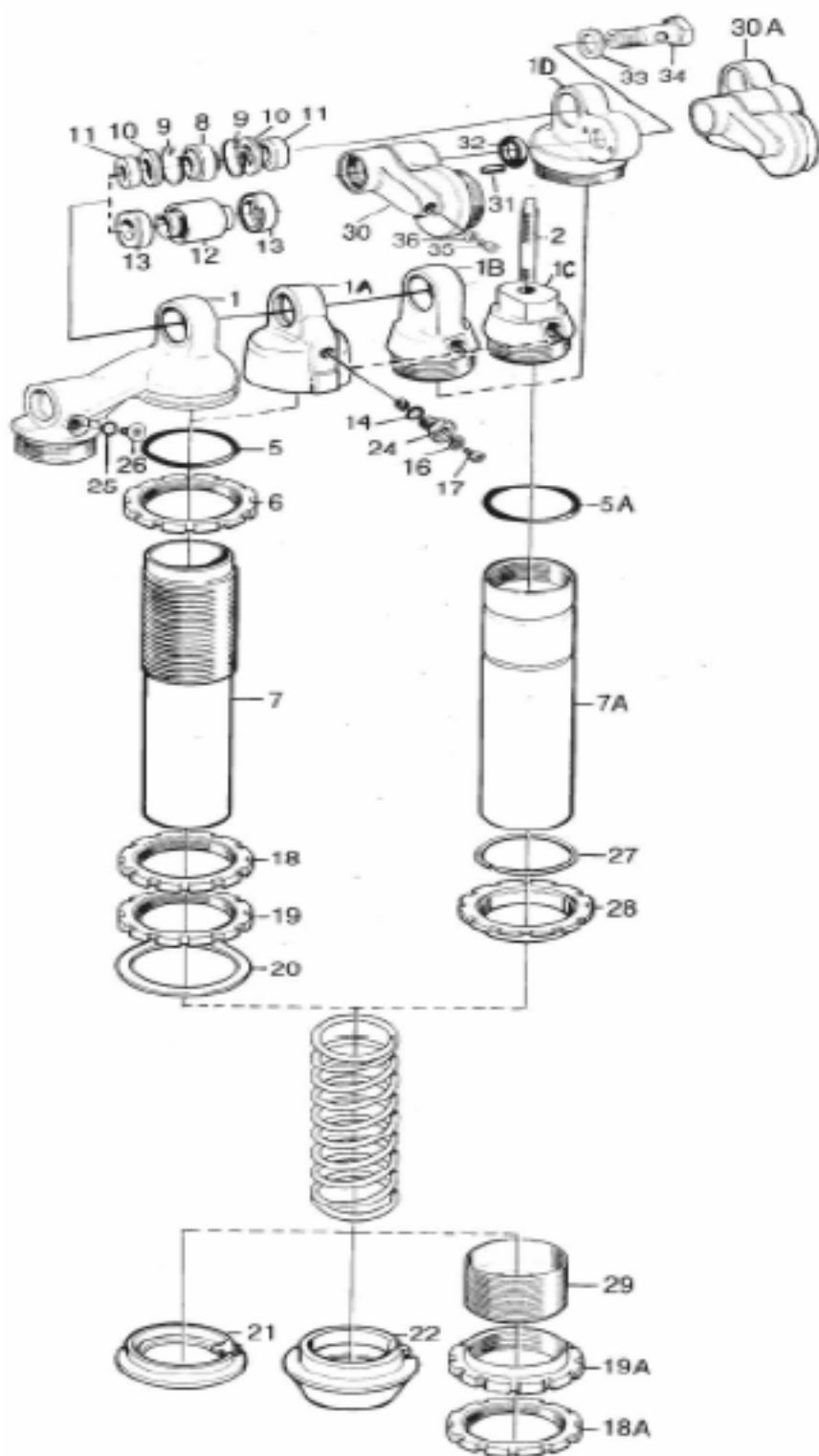
Fig.2 Cylinder head/tube
